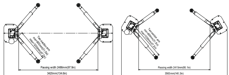
Symmetric installation
